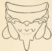
FIG. 18.—HOLOTELSON TUBERCULATUS. ABDOMEN OF MALE. \times 3\frac{1}{2} .
